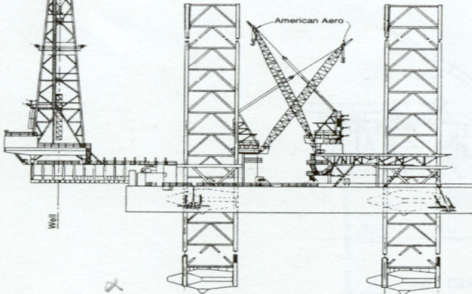
Outboard Profile
